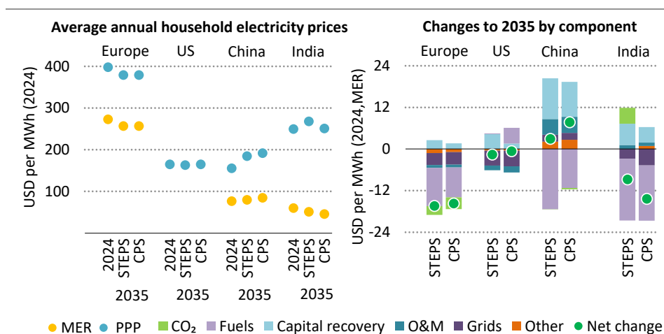
Figure 5.38 ▶ Household retail electricity prices in selected country/region by scenario, 2024 and 2035, and by contributing factor in 2035
