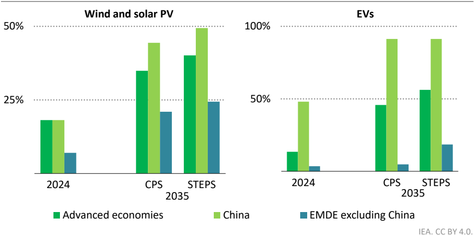
Figure 1.33 ▶ Wind and solar PV in total generation and market share of EVs in car sales by region and scenario, 2024-2035
