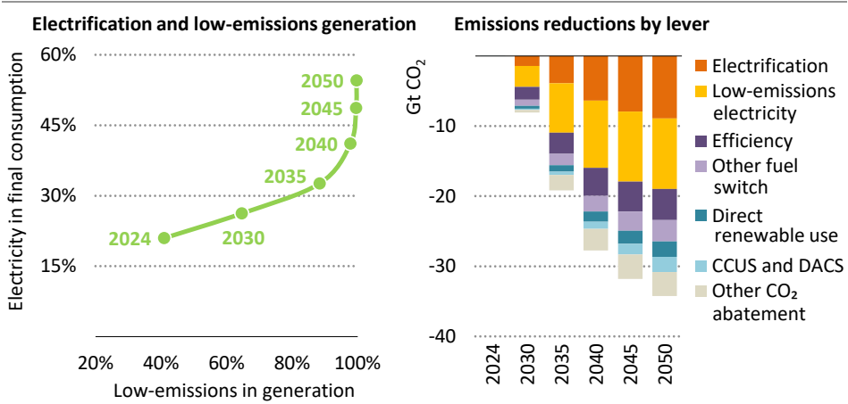
Figure 7.12 ▶ Low-emissions share of generation relative to electricity in final consumption and levers employed to cut emissions in the NZE Scenario, 2024-2050
