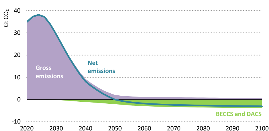
Figure 7.8 ▶ Global gross and net energy-related CO 2 emissions in the NZE Scenario, 2020-2100
